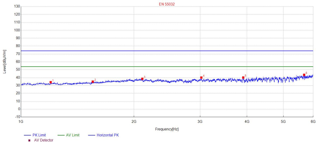
Test graph and data for Radiated Emission Above 1GHz at Horizontal
